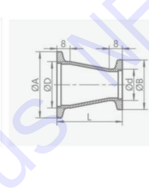
真空法兰式大小头 / KF Concentric Reducer
