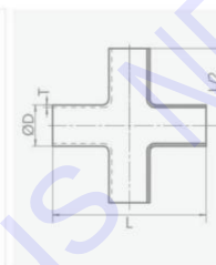
焊式等径四通 / Weld 4 Way Equal Cross
